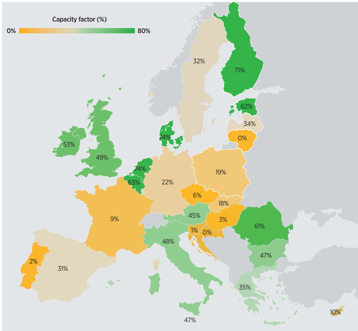
Figure 23: Average capacity factors for combined-cycle gas plants by EU Member State in 2030 under REmap
